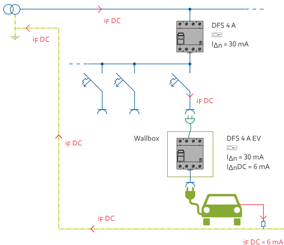
Residual current protection for charging – schematic diagram
