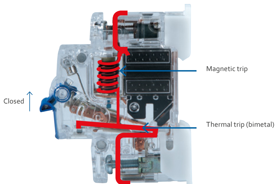
Overcurrent protective equipment, circuit-breaker, structure
